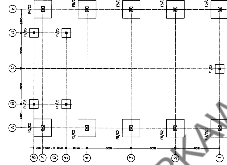
PAD FOOTING KEY PLAN
