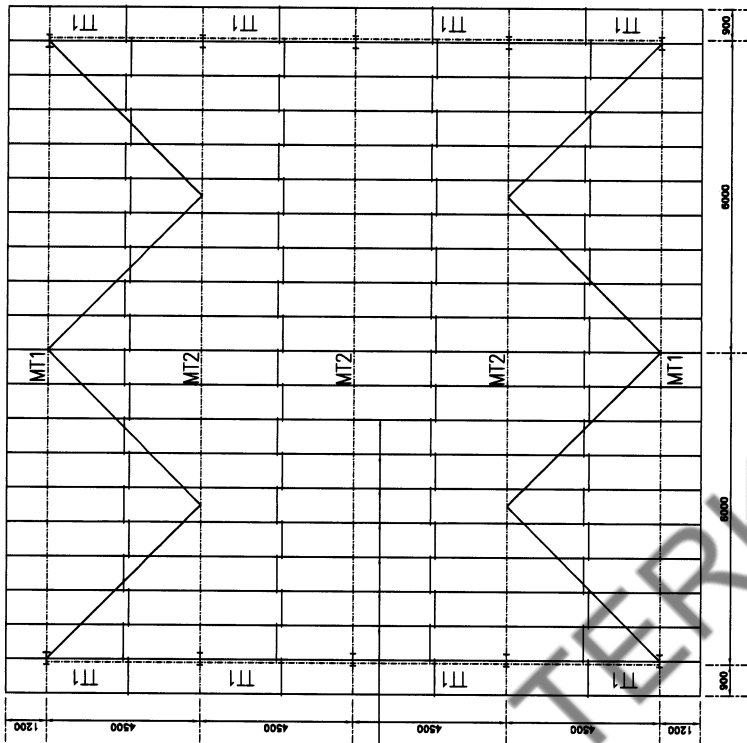
ROOF TRUSS LAYOUT PLAN
