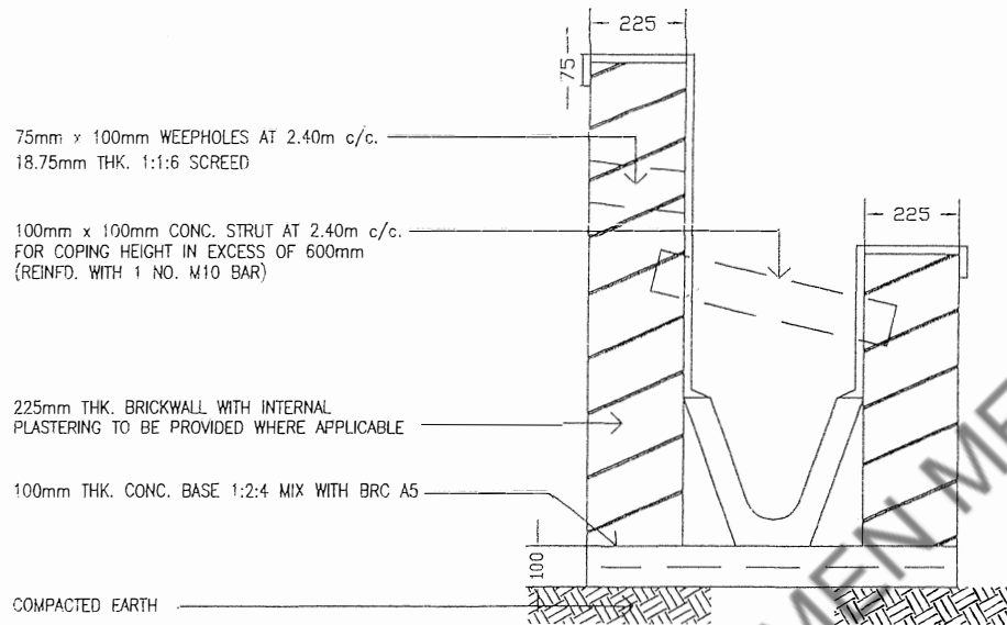
TYPICAL V-SHAPE SECTION
