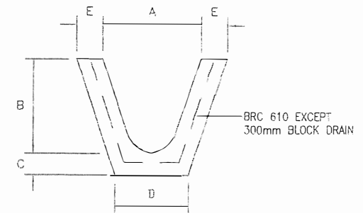
TYPICAL SECTION OF CONC. V-SHAPE
