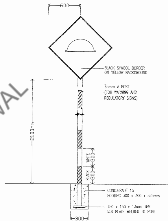
PLACEMENT OF SIGN SCALE :- N.T.S
