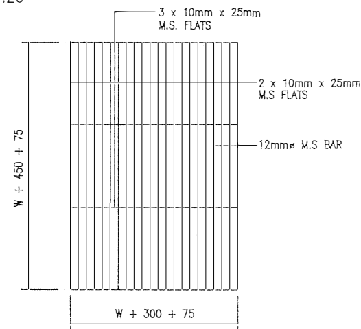
PLAN VIEW OF GRATING
